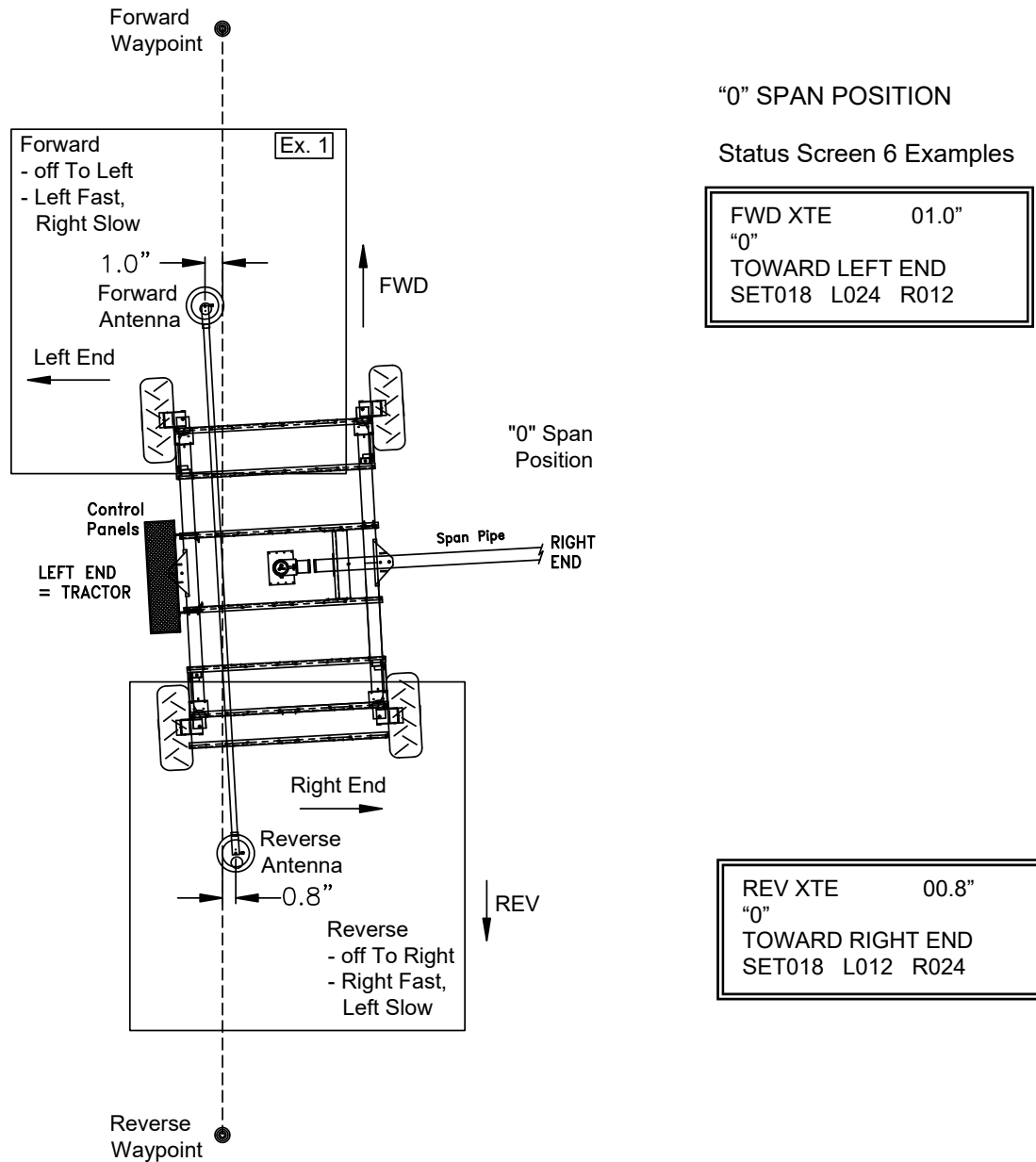
Figure 26. GPS Navigation Steering – Ultra G2 "0" Span Position.
