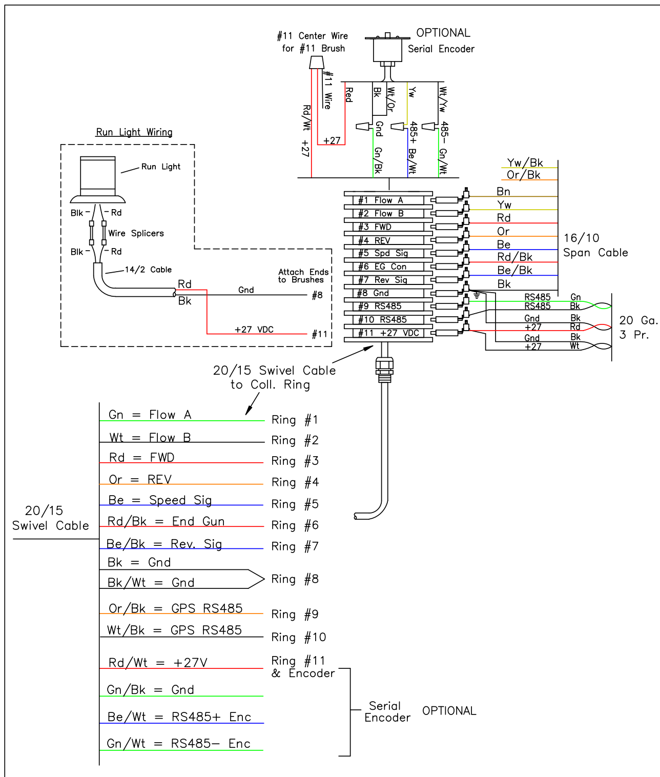
Figure 20. Wiring of ULTRA G2 with GPS Navigation at Center.
